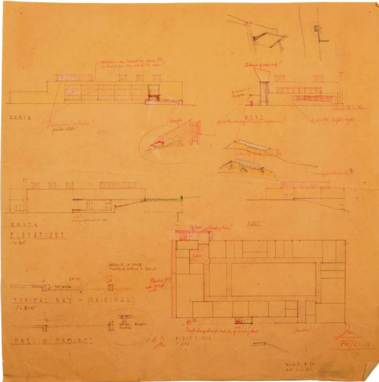
Erich Mendelsohn, Atomic Energy Building, UC Berkeley, Preliminary Project Drawings to Scale, 1952 Pencil on heliographic paper, 18 1/8 x 18 1/8 in. (46 x 46 cm) EMEN006, •
